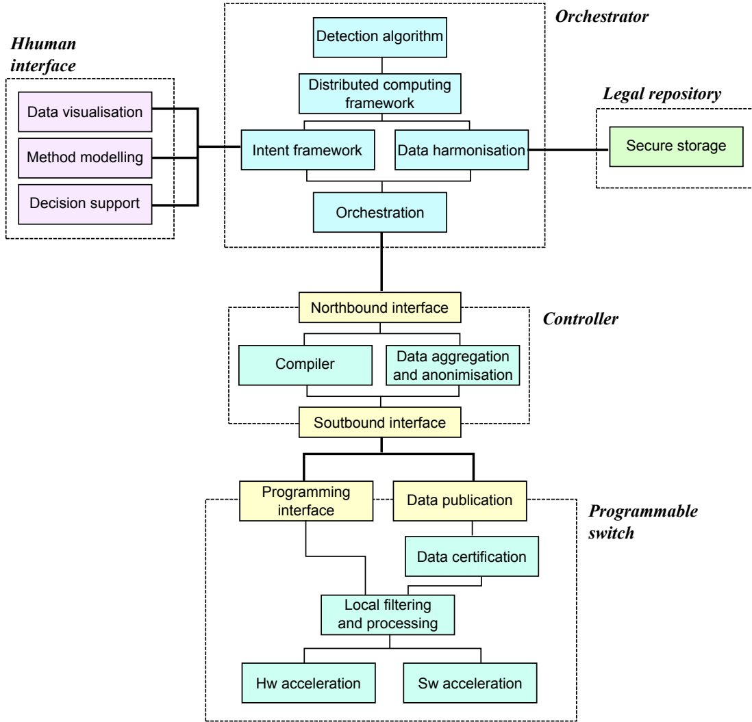
Figure 4: Reference platform design
